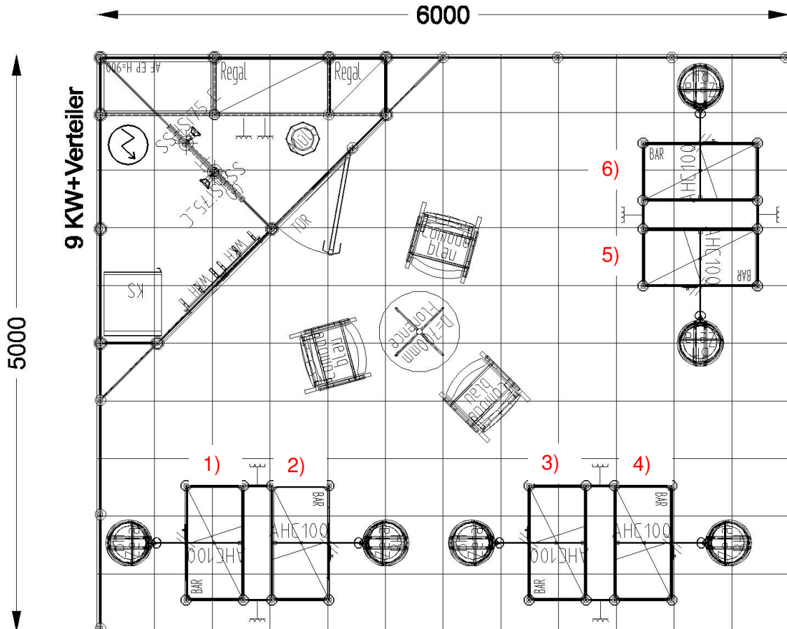
picture 3) COMPOSITES EUROPE WPC/ NFK Pavillon – plan view; 6 workstations
